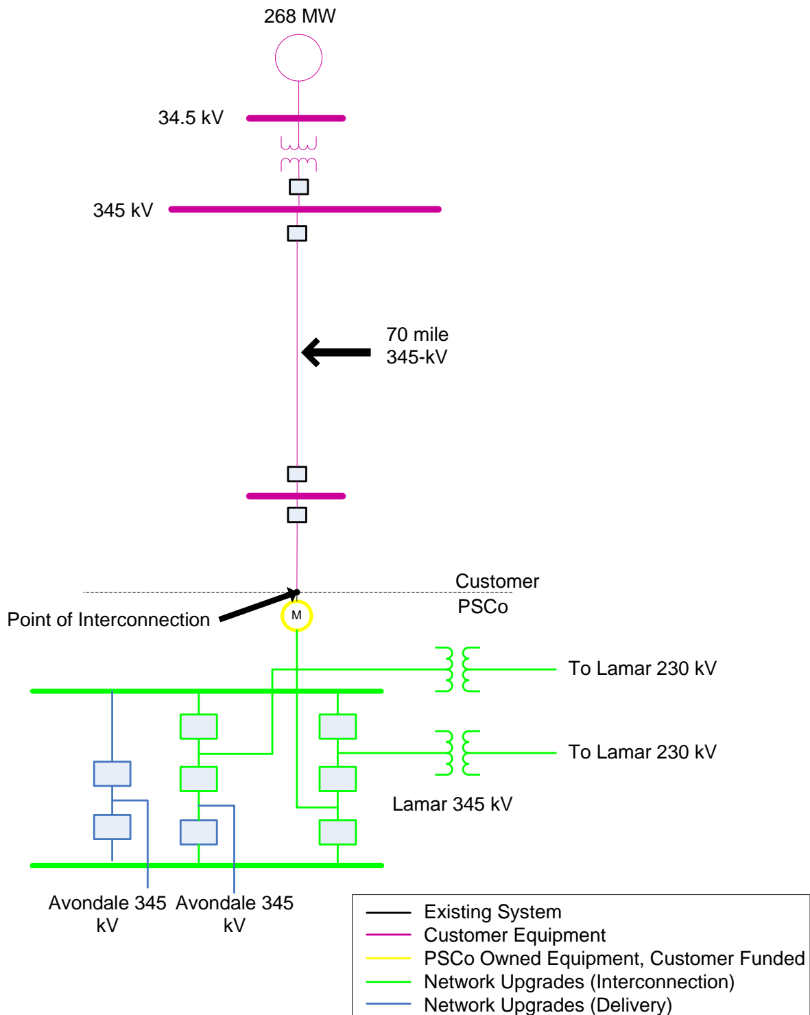
Figure 1 Preliminary One-Line of the Proposed GI-2010-2
